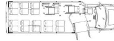
28', 16+4 Passenger, 2 w/c
