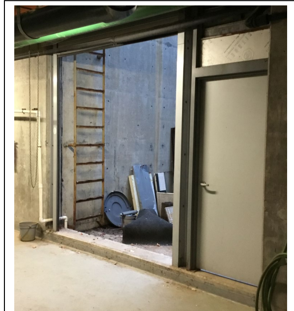
Figure 004 – Areaway access from filter room
