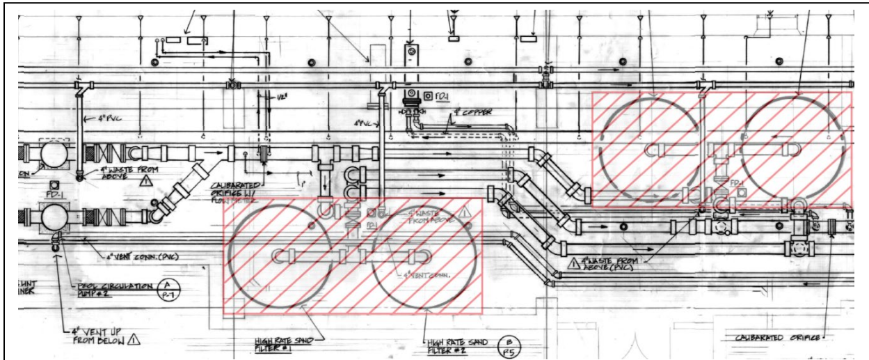
Figure 001 – Demolish existing sand filter tanks, valves, and face piping.
