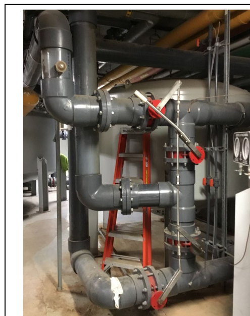
Figure 003 – Existing face piping (typical)
