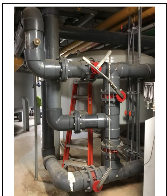
Figure 003 – Existing face piping (typical)
