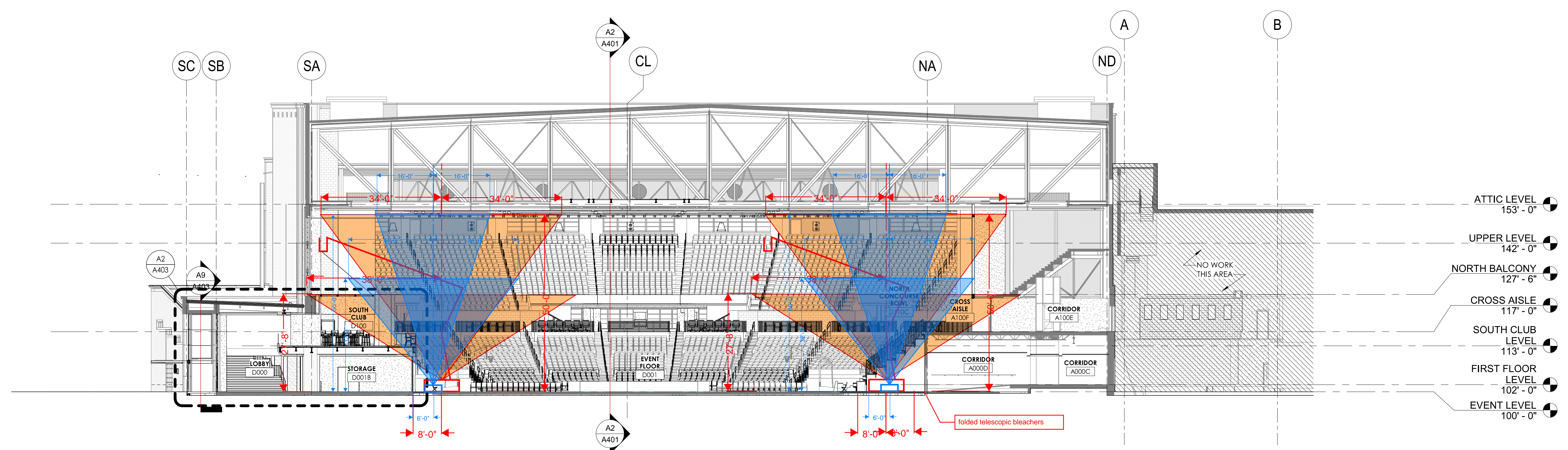
OVERALL SECTION - NORTH/SOUTH E2 1/16" = 1'-0"
